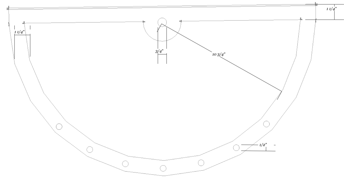
A BRACKET DETAIL 001
